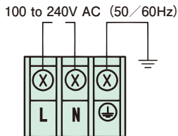
③ : Power supply terminal
