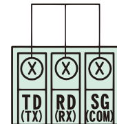
⑥ : RS-232C Communication terminal
